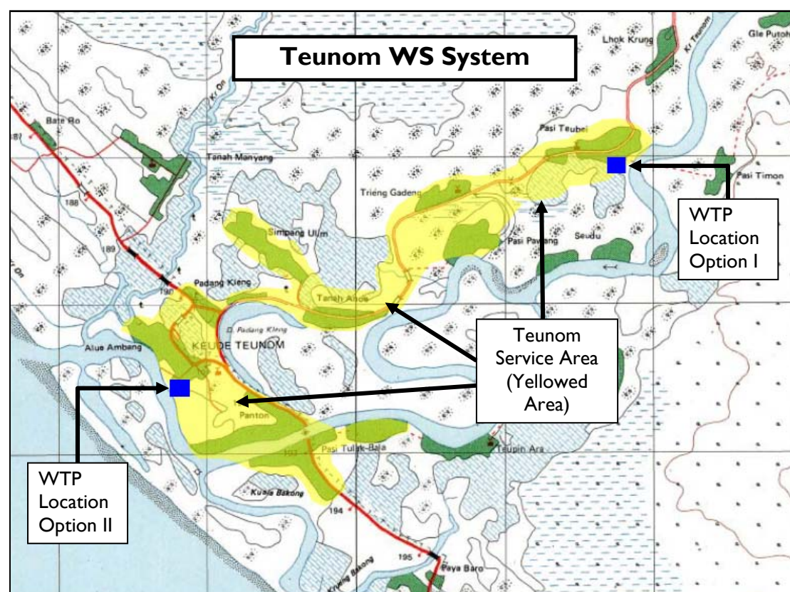
Figure 12: Teunom Water Supply
