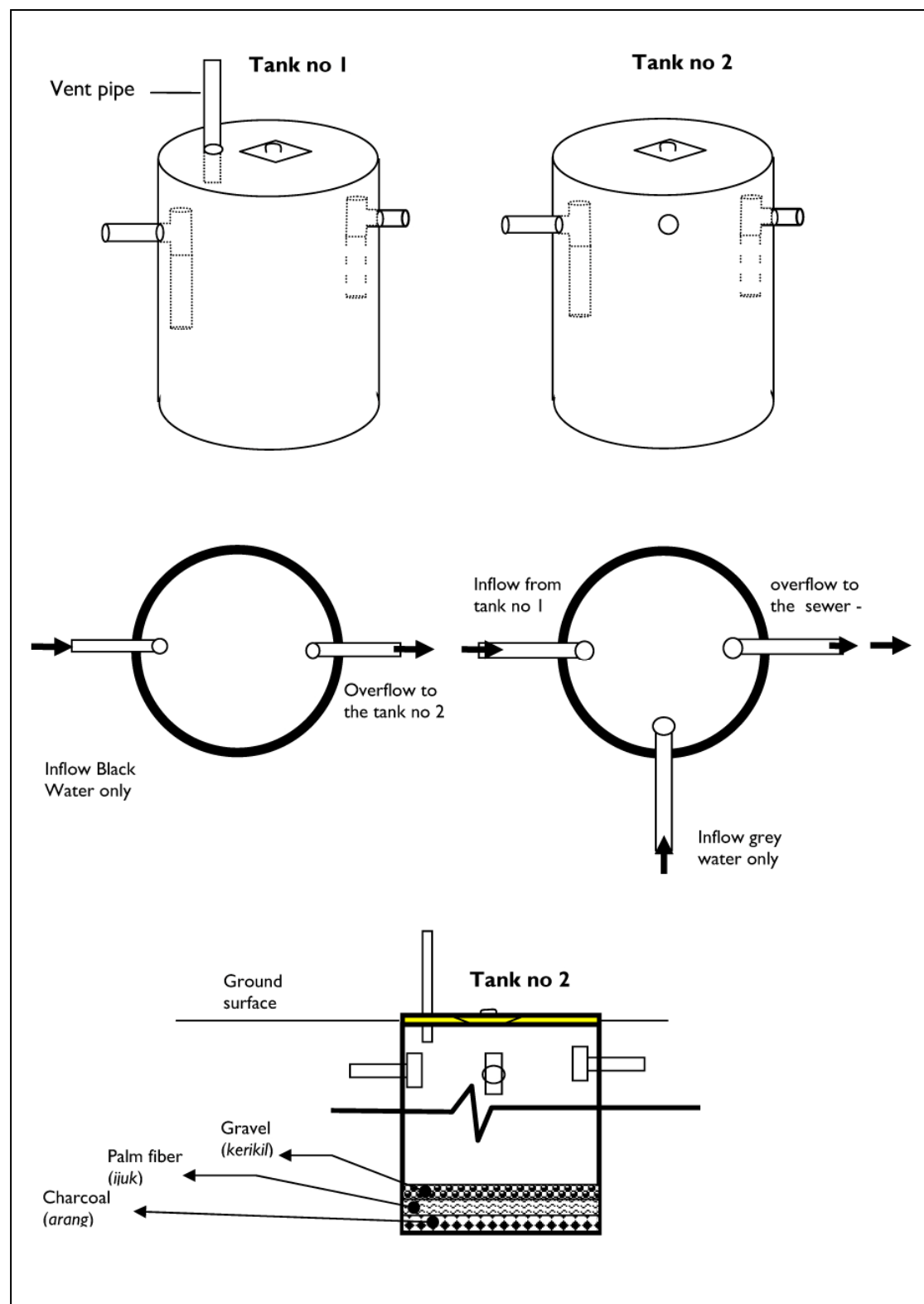
Figure 6: Typical Two Tanks Septic System
