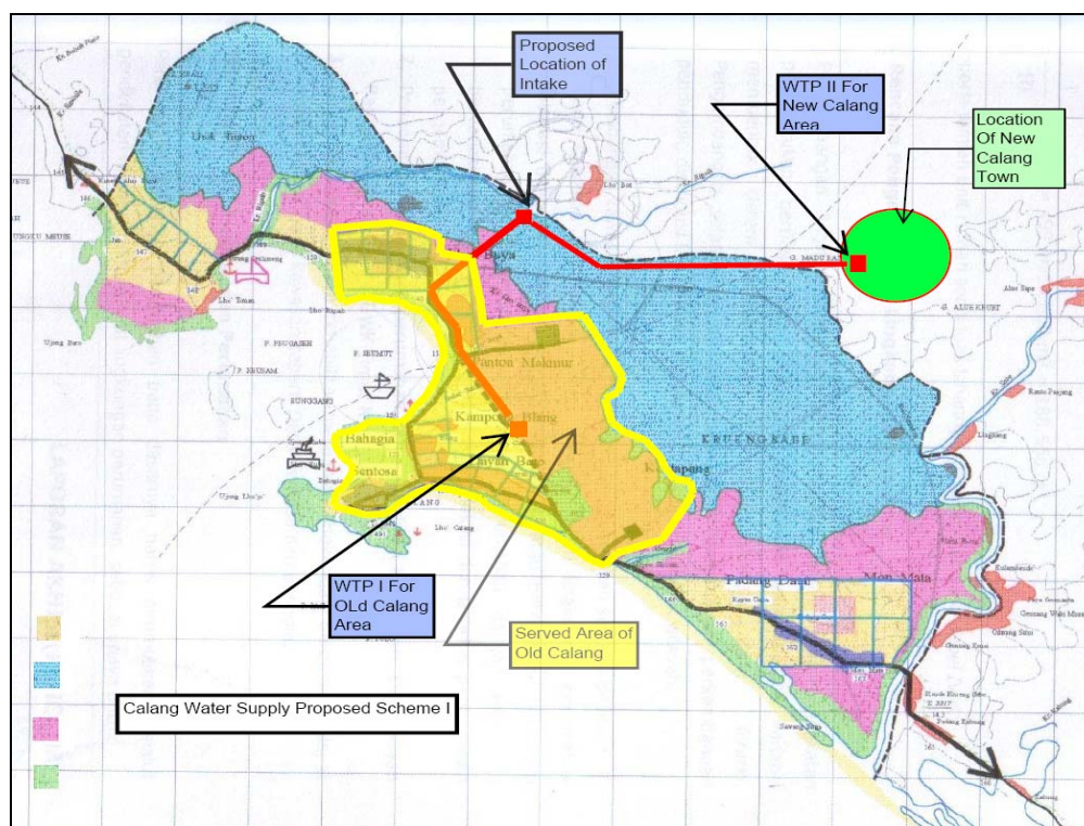
Figure 10: Calang Water Supply from Kr. Bot (Rigah)
