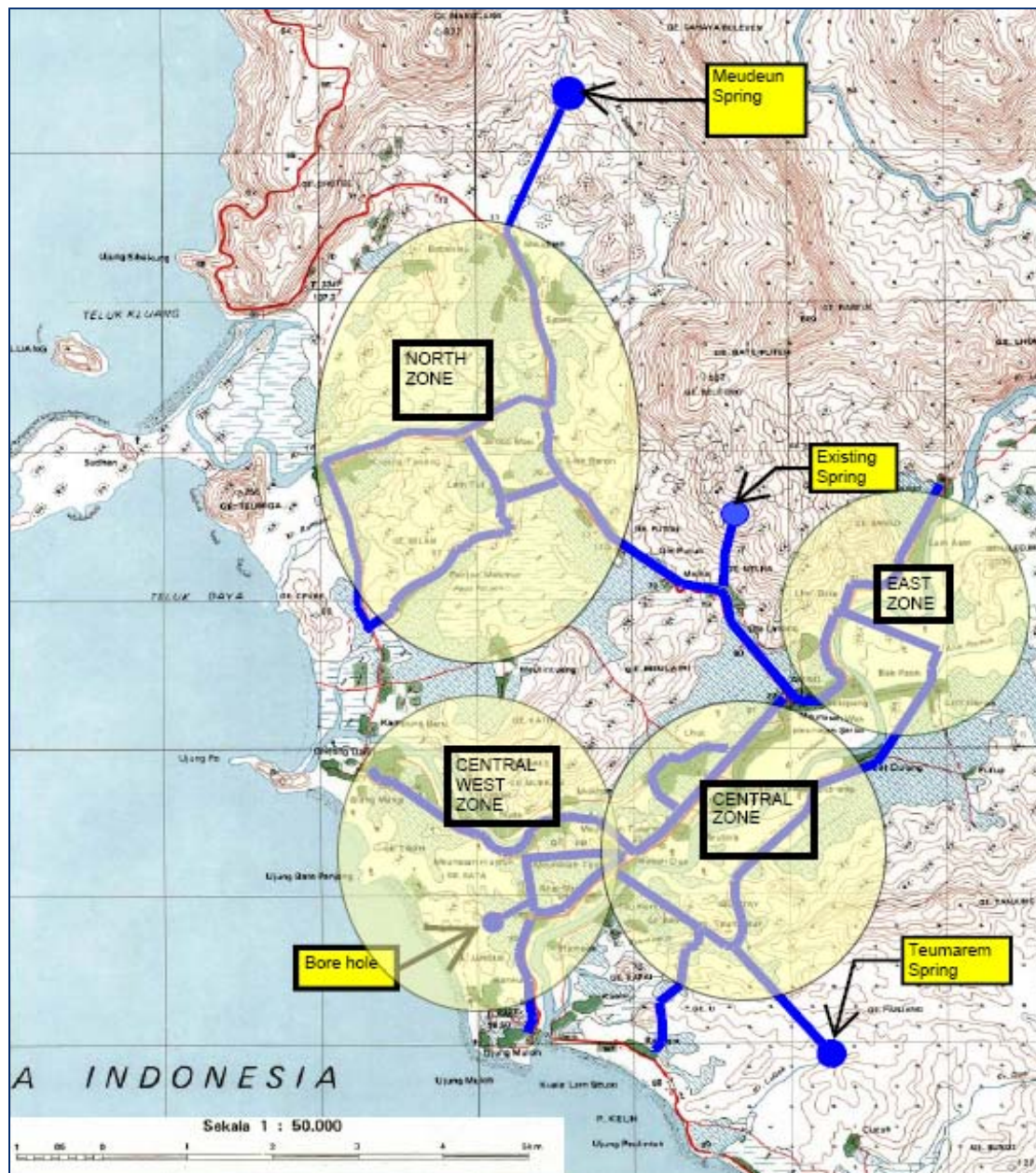
Figure 8: Lamno Water Supply Scheme (by OXFAM)
