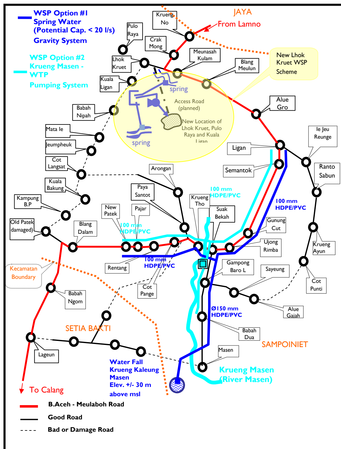
Figure 9: Sampoiniet Water Supply Scheme
