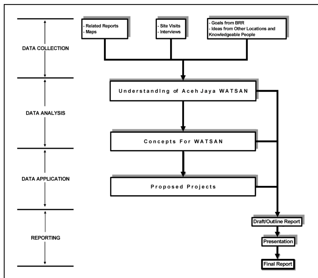
Figure 1: Methodology
