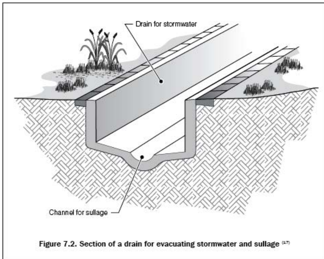
Figure 19: Combined Sullage and Stormwater Drain
