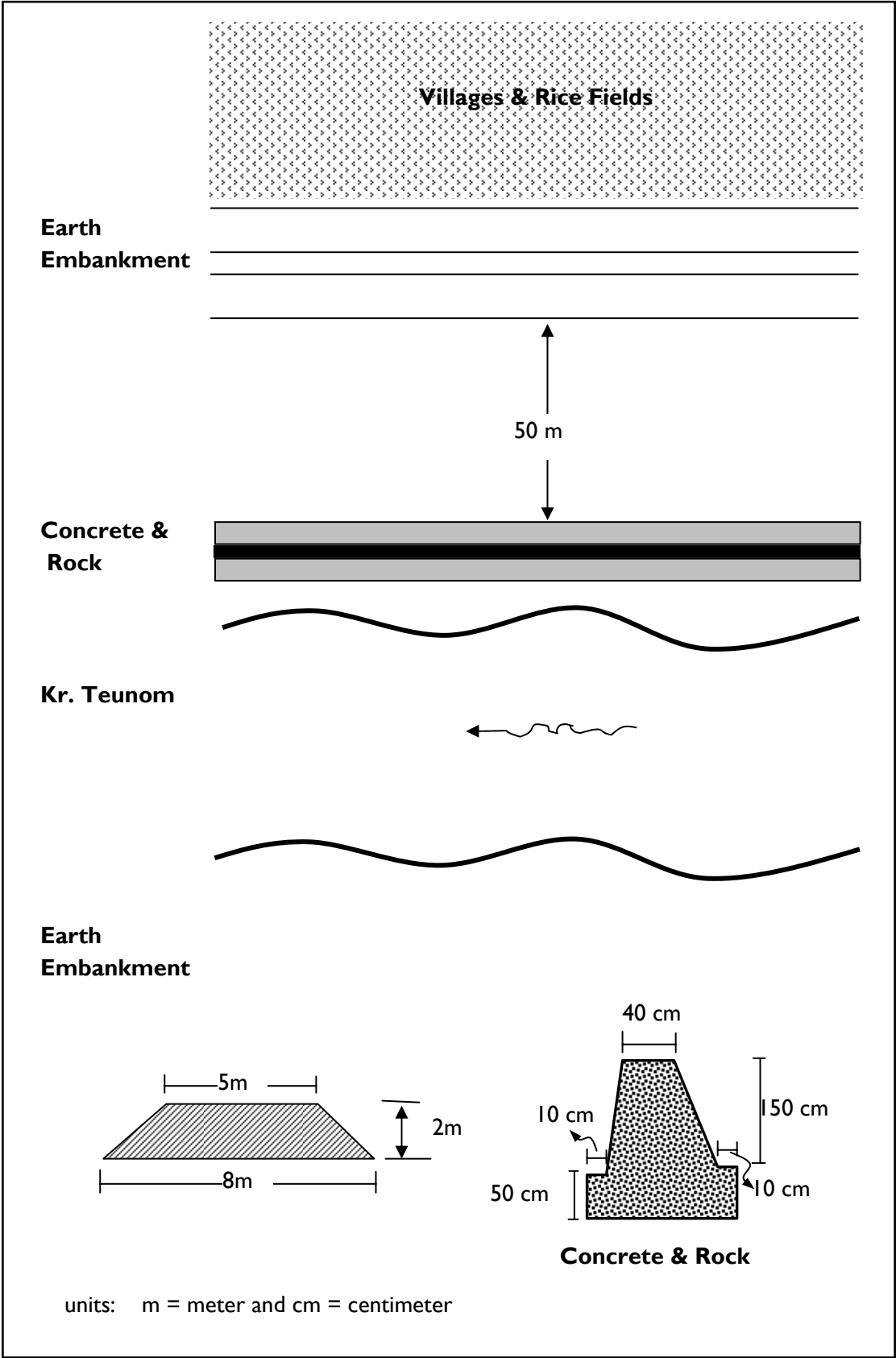
Figure 9: Krueng Teunom Embankment Sketch
