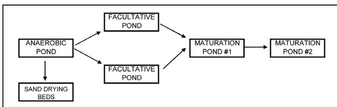
Figure 7: Flow Scheme for IPLT Stabilization Ponds
