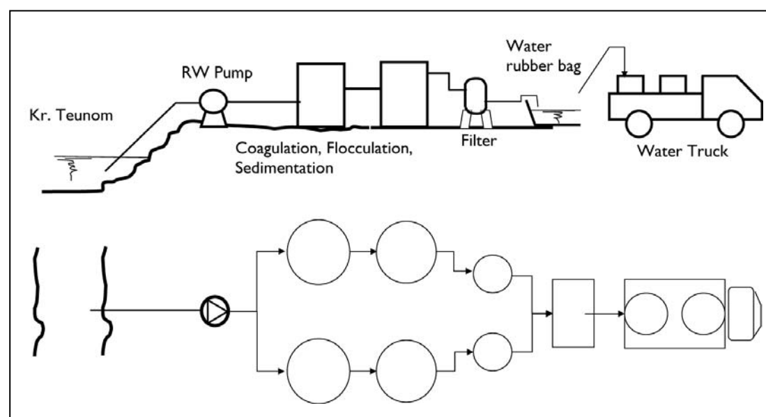
Figure 6: Sketch of German Red Cross Water System in Teunom
