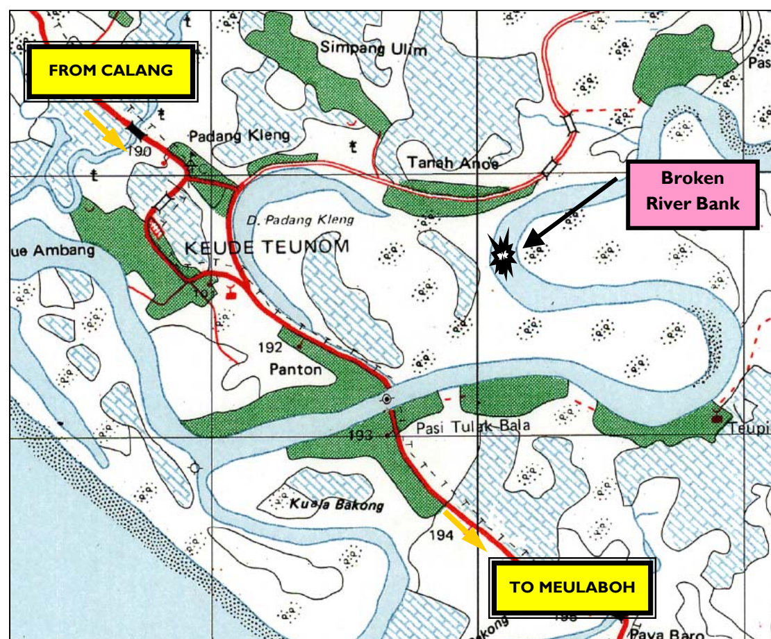
Figure 8: Krueng Teunom River Embankment Break
