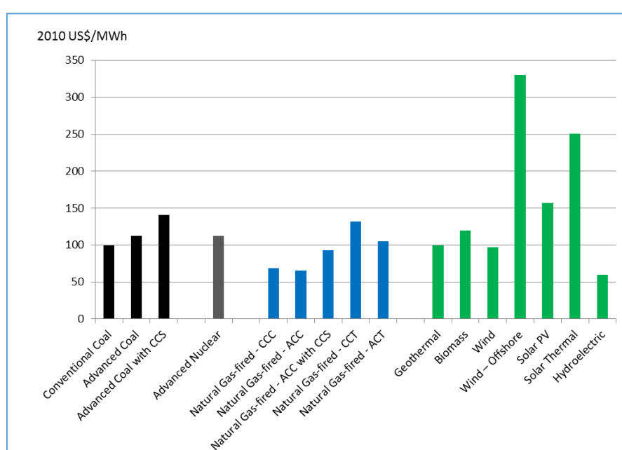
Figure 13: US average levelized costs of electricity by technology, 2010 USD/MWh
