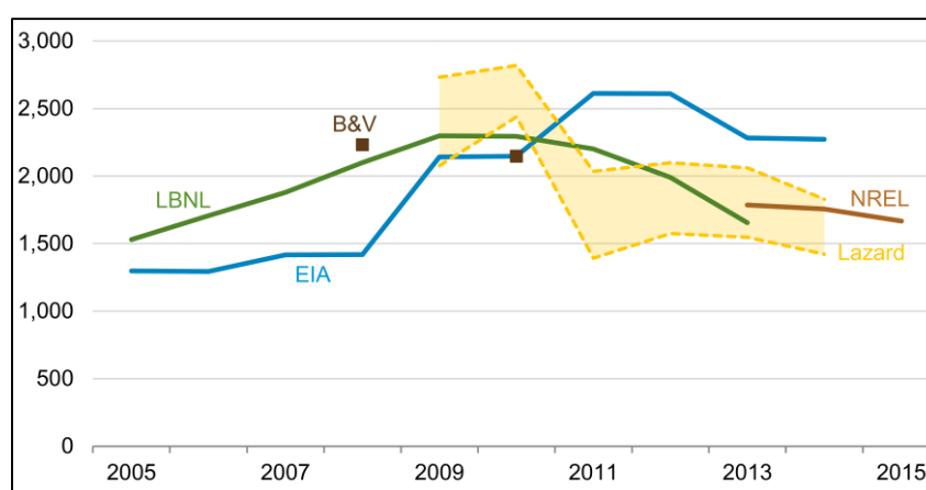
Figure 12: Annual estimated capital costs for wind technologies from various agencies, 2005-2015 (in 2014$ per kilowatt)
