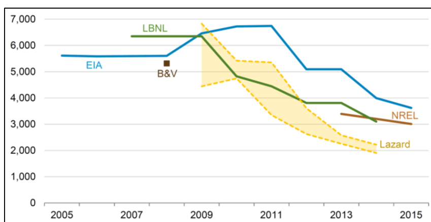
Figure 11: Annual estimated capital costs for solar PV technologies from various agencies, 2005-2015 (in 2014$ per kilowatt)
