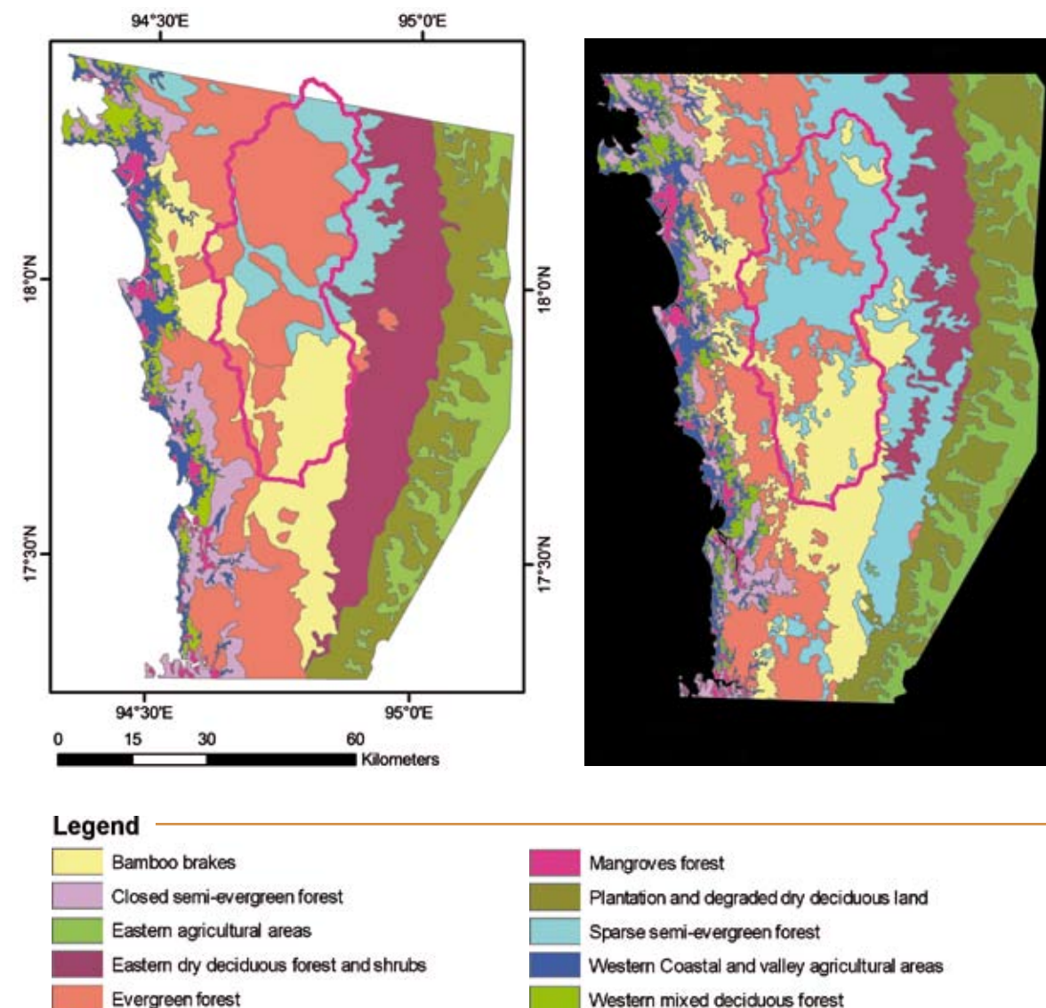
Land cover map of Rakhine area 1974 (left) and 2000-2003 (right)
