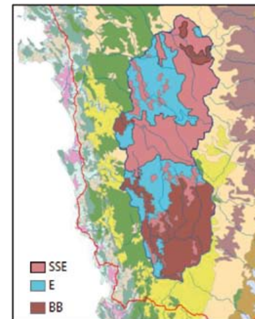
NDVI changes for land cover (2000) within the Rakhine Yoma Elephant Range WR
