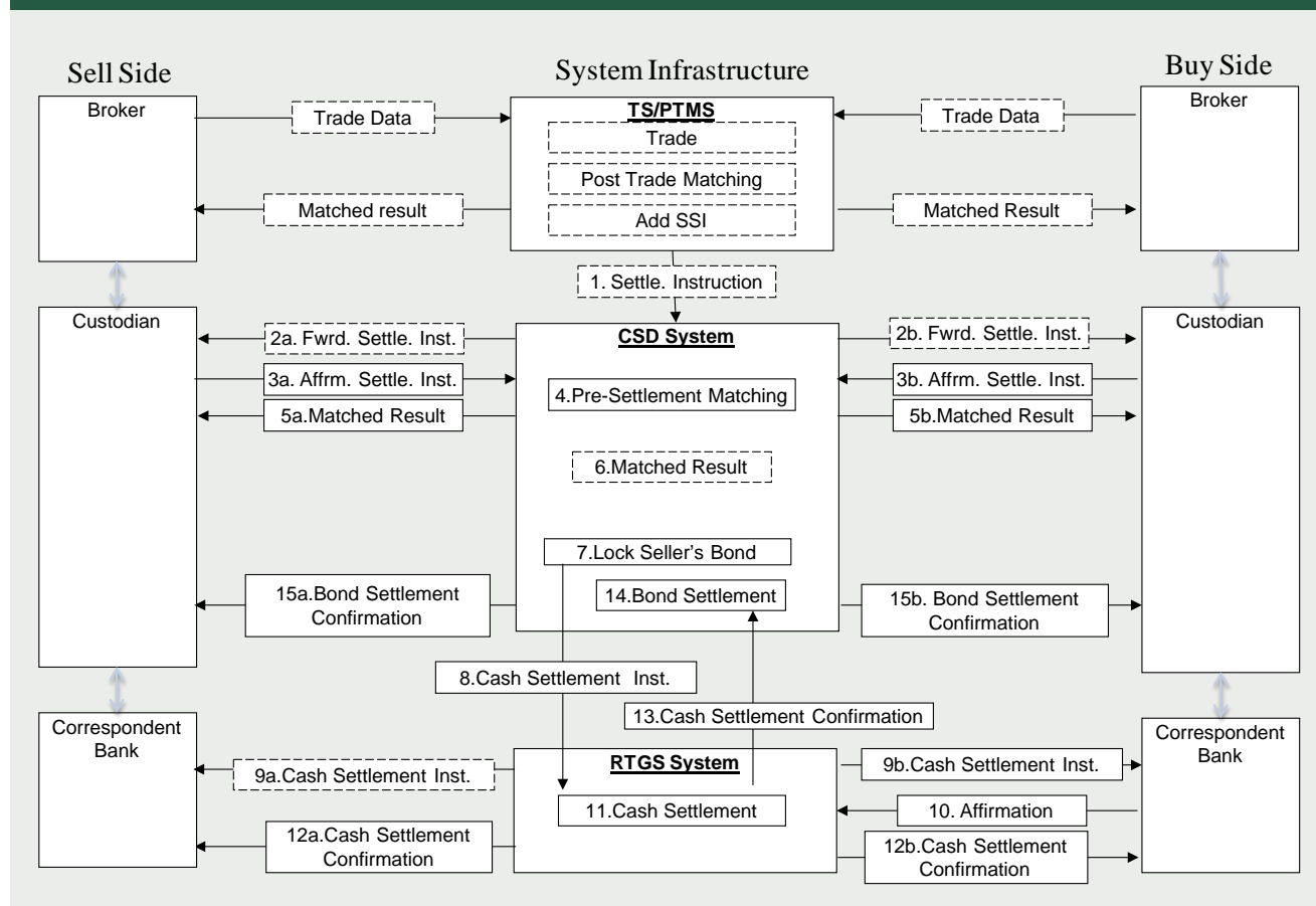
Figure 6.3 Draft Reference Model DVP Flow (Central Matching without PSMS)
