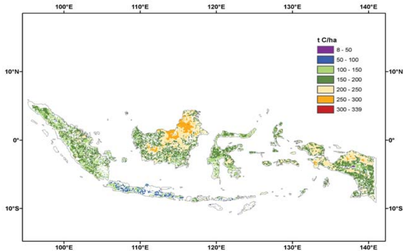
Figure 4. Above and below ground carbon stocks in Indonesia
