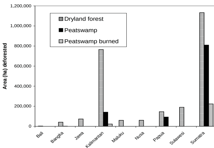
Figure 8. Area of dryland and peat swamp forests deforested during 2000-2005 by Island.
