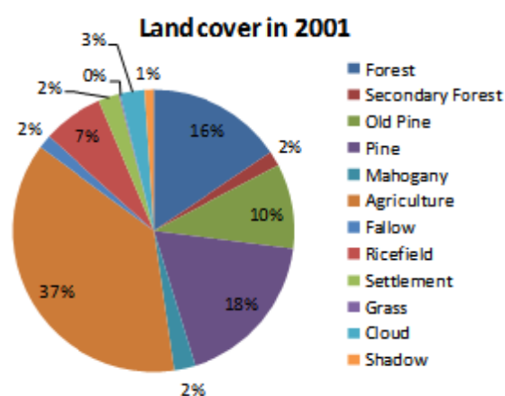
Figure 9. Land-cover classes in the KFR, 2001.
