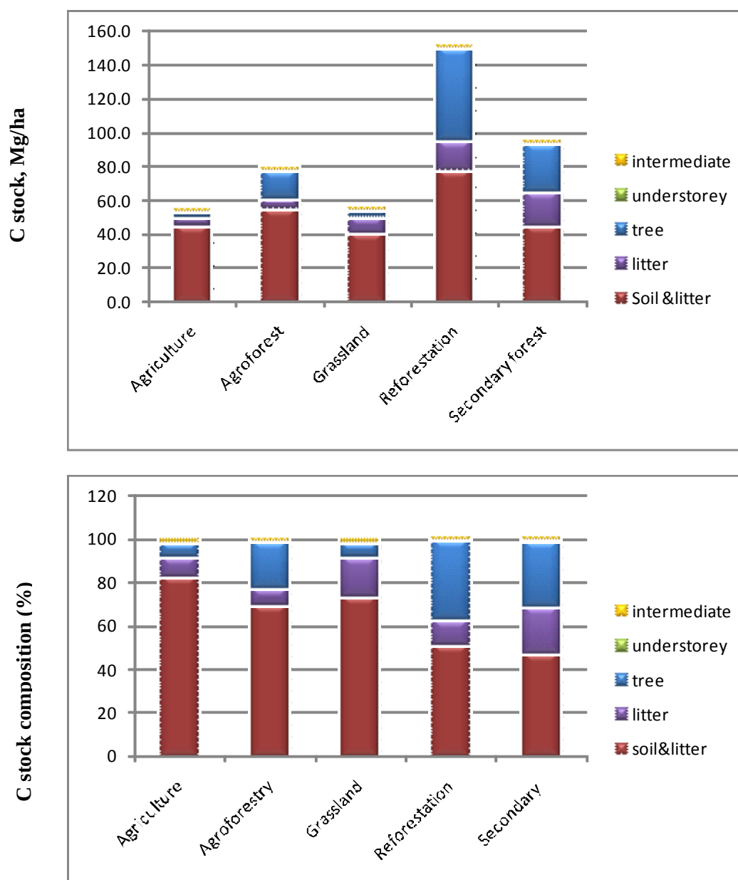
Figure 5. Total (above- and belowground) carbon stocks and their relative composition in the KFR (Upper panel: absolute values in Mg/ha. Lower panel: as percentage).
