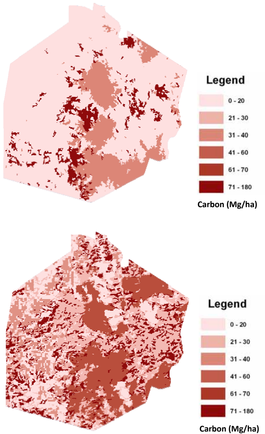
Figure 12. Distribution of land-cover-derived carbon density in the KFR in 1989 ( upper panel ) and 2001 ( lower panel ).
