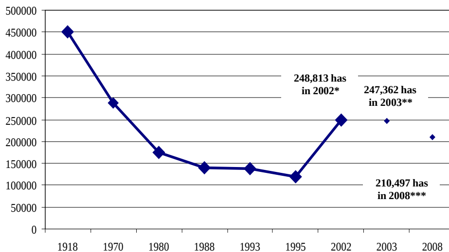
Figure 16. Trend in mangrove cover from 1918 to 2008.
