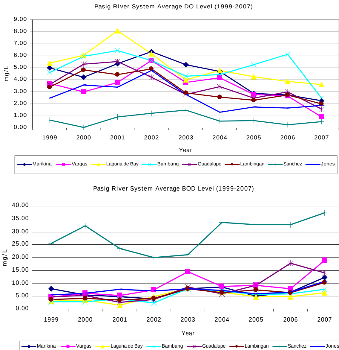
Figure 13. Average DO and BOD levels in Pasig River System 1999 -2007 (EMB, 2007).
