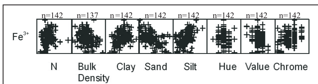
Figure 22. Scatters of measured \text{Fe}^{3+} versus visible soil characteristics (Munsell hue, value, chrome) (For units see text)
