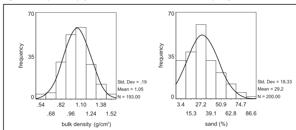
Figure 7. Example of soil physical data with normal and non-normal frequency distributions
