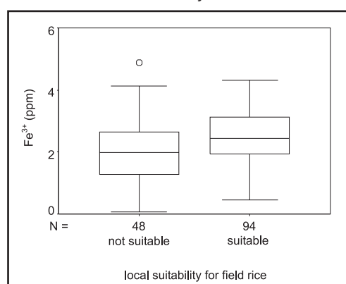
Figure 21. \text{Fe}^{3+} as variable to discriminates classes of farmer's suitability assessment for rice
