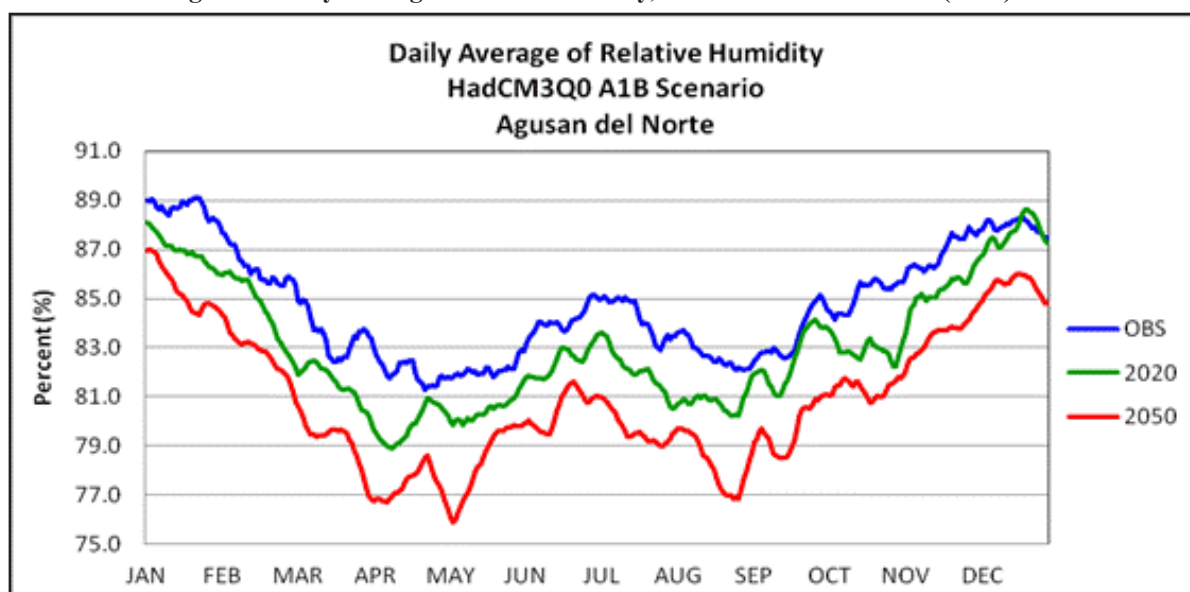
Figure 5: Daily Average Relative Humidity, PAGASA Butuan Office (2010)
