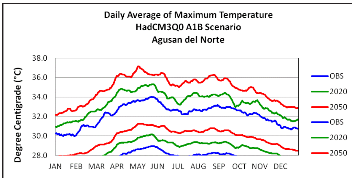
Figure 4: Daily Average Maximum Temperature, PAGASA Butuan Office (2010)
