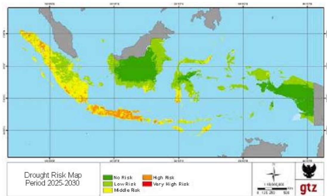
Figure 7 Drought Risk Areas based on Scenario SRA2 for 2025-2030
