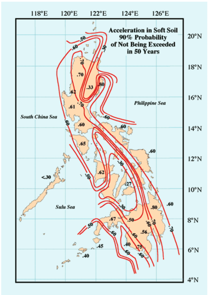
Figure A3.1 Peak Ground Acceleration (PGA) Value for Soft Soil
