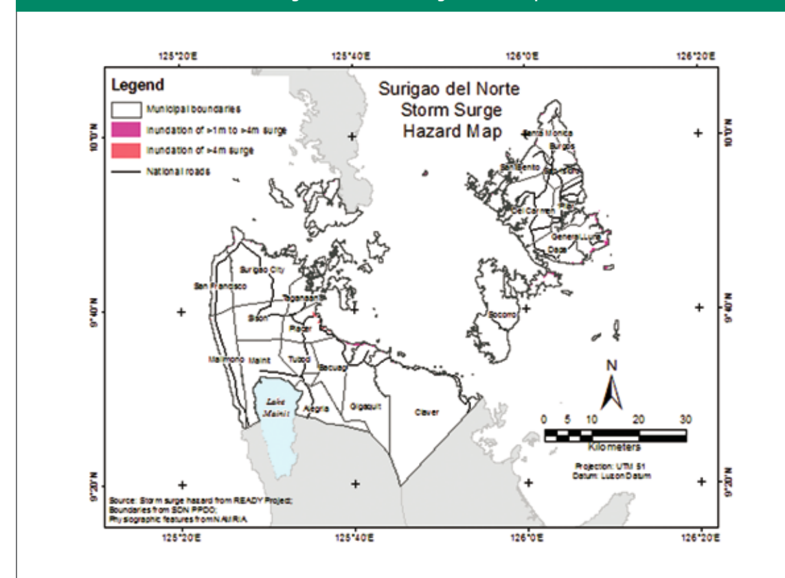
Figure A1.9 Storm Surge Hazard Map
