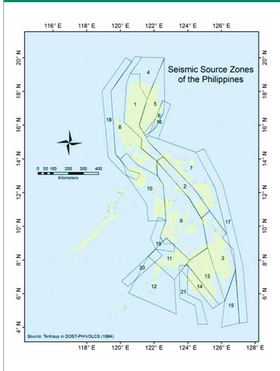
Map 3 Seismic Source Zones of the Philippines
