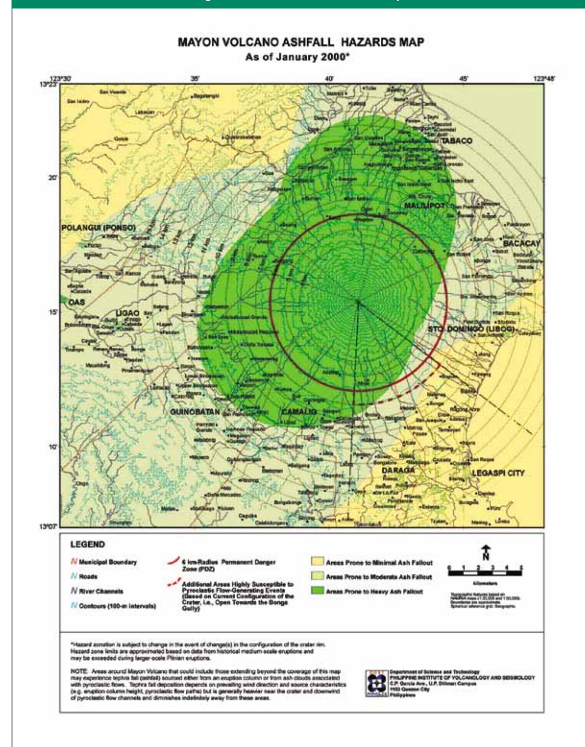
Figure A1.8 Volcanic Ashfall Hazard Map
