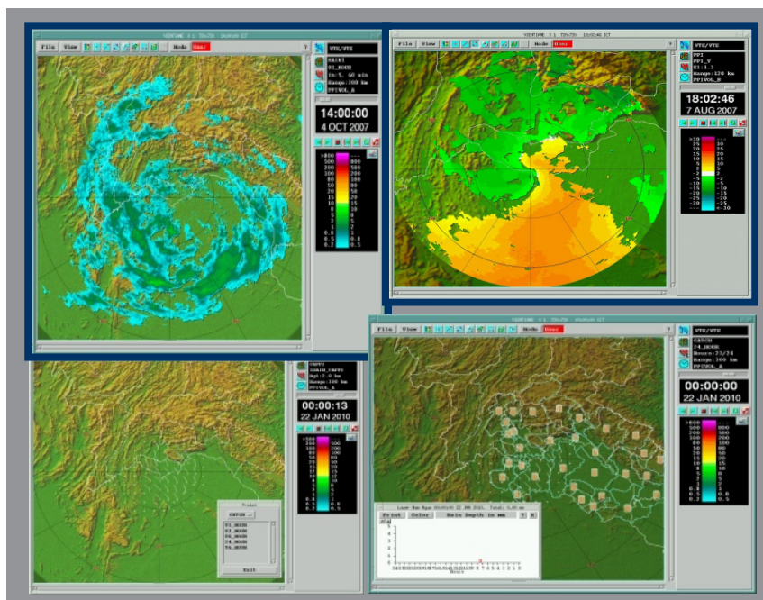
Figure 8.1 Radar image showing estimated
