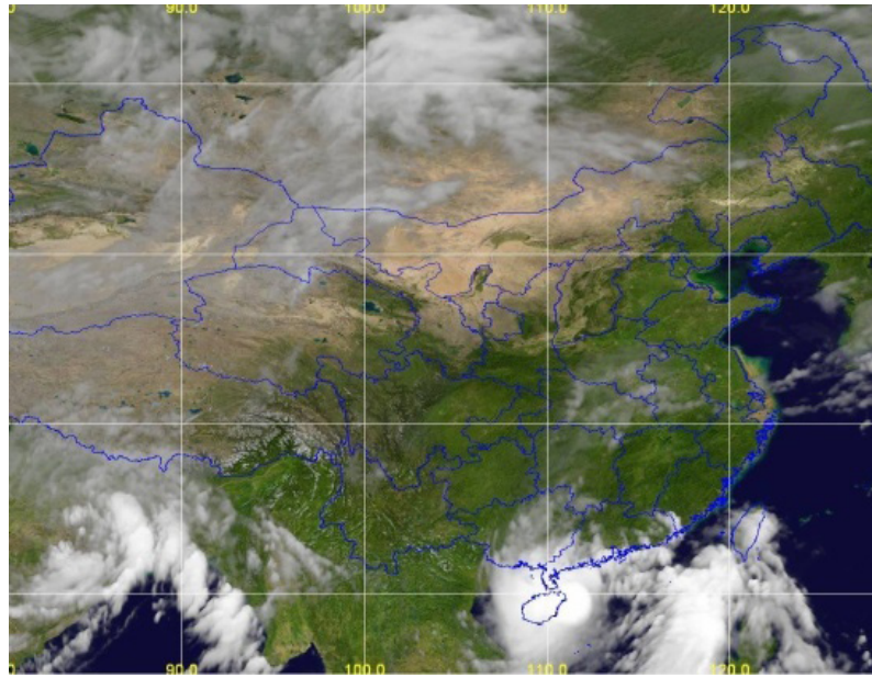
Figure 8.2 Satellite image (MTSAT)
