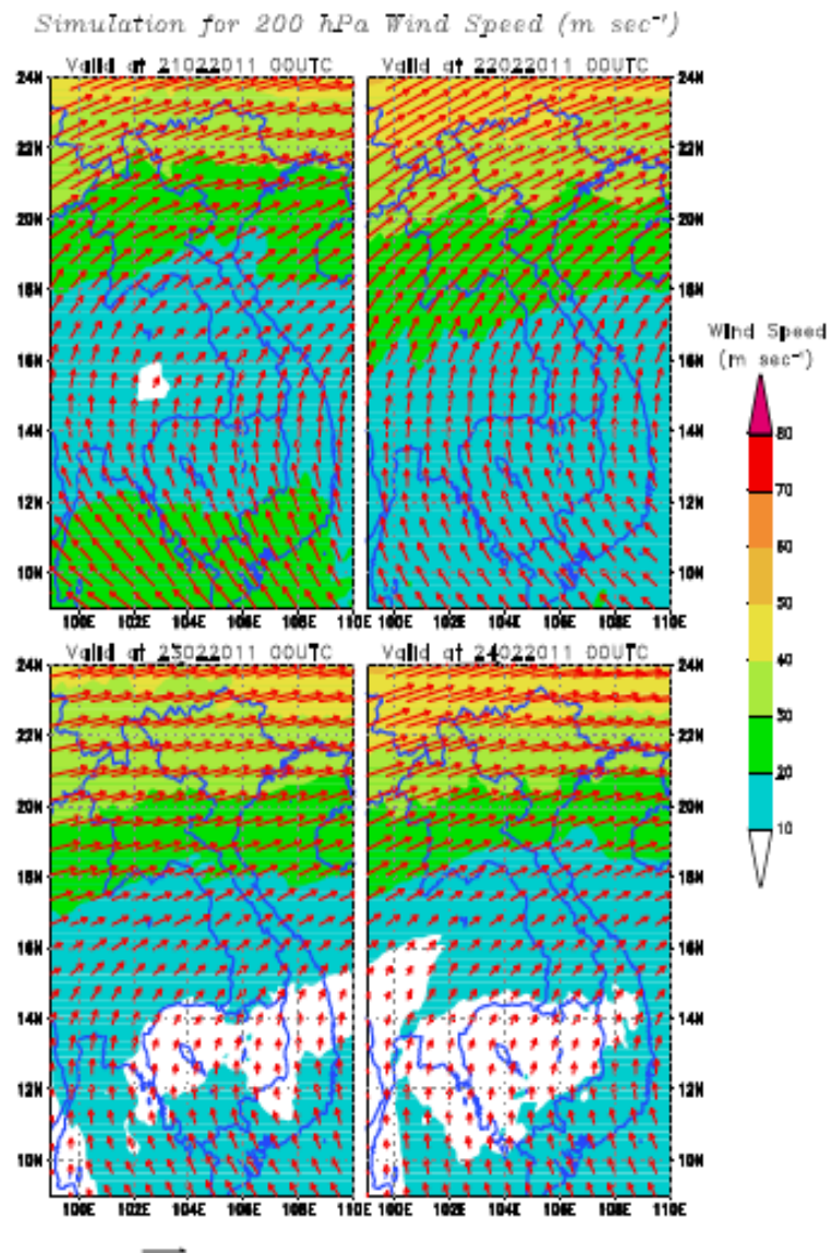
Figure 8.3 Wind at 200 hPa product of RIMES
