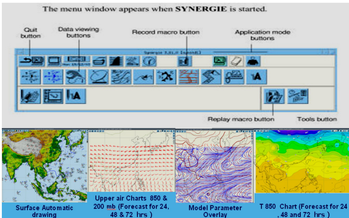
Figure 9.3 NWP products from ECMWF for Severe Weather monitoring and forecasting in Laos using Synergie Version 3.4.0
