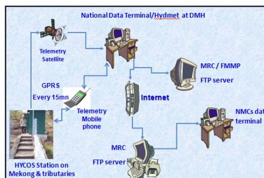
Figure 6.8 MRC Hydrological Cycle Observation Stations (HYCOS) in the left figure and data acquisition system in the right
