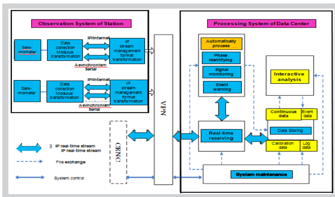
Figure 9.2 Topology of the Data Center
