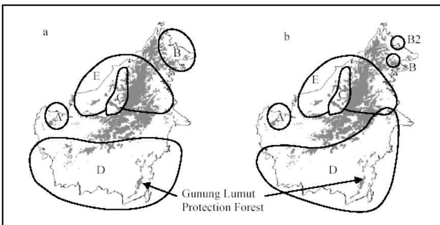
Figure 14. Floristic relations within Borneo based on (a) steinhouse similarity and (b) sorensen similarity of 28 locations across Borneo
