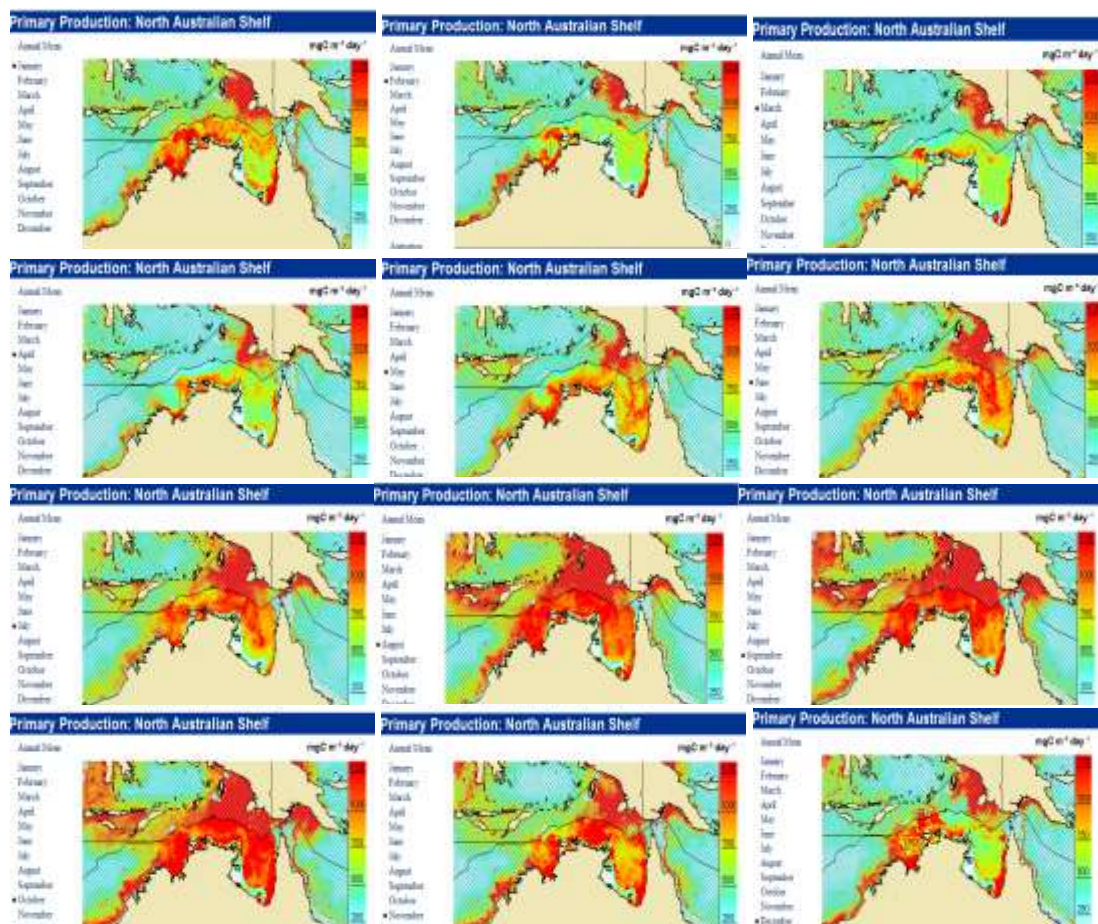
Figure 11. Estimated monthly primary productivity ( \text{mgC m}^{-2} \text{day}^{-1} ).
