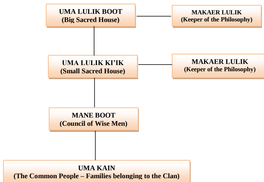
Figure 8. Clan Structure
