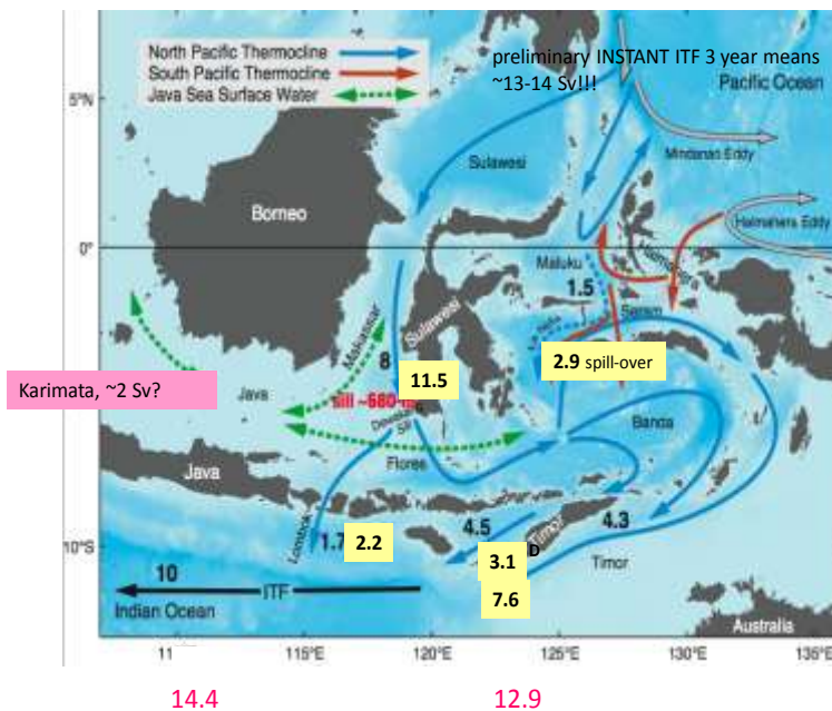
Figure 7. Summary of Indonesian Through Flow. Arrows indicate ocean current through Indonesian straits. Numbers are current in Sverdrups.
