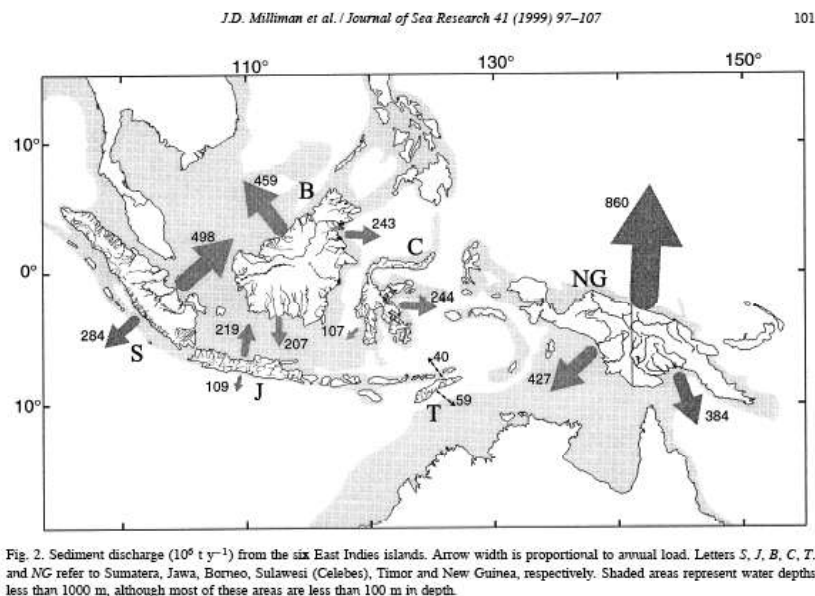
Figure 2. Sediment discharge ( 10^6 \text{ t yr}^{-1} ) from the six East Indies islands. Arrow width is proportional to annual load (Milliman et al. , 1999).
