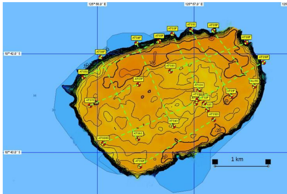
Figure 29. ATSEA Shoal – towvideo transect nominal locations marked as green dashed lines, between start and end waypoints, in relation to the interpolated, acquired single-beam bathymetry of the shoal plateau down to the 60m depth contour. The acquired bathymetry is superimposed on the available chart bathymetry, revealing significant inconsistencies.
