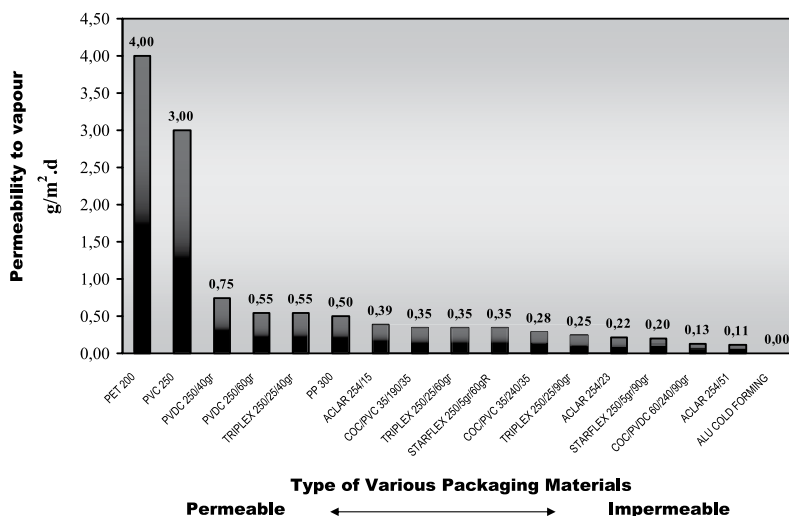
Figure 1 Permeability to Vapour of Various Packaging Materials (Method ASTM F1249, 38°C/90%RH)
