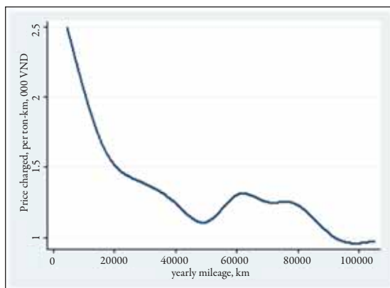
Figure 2.10 Unit trucking price per ton-km by a truck's yearly mileage, one trip distance, and truck size
