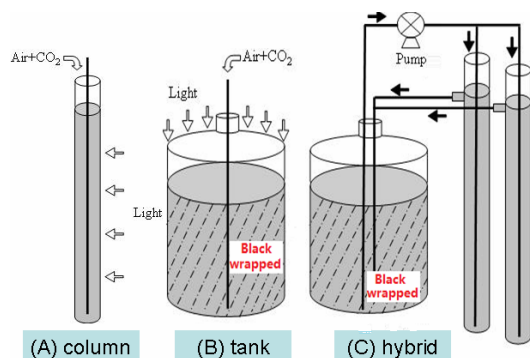
Fig. 1: Schematic graph for indoor cultivation
