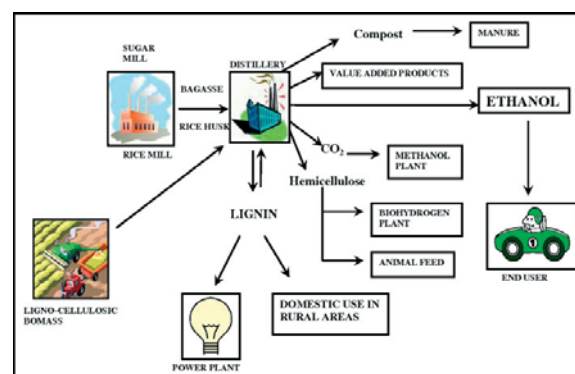
Fig 4: Process integration/industrial complexing opportunities for ethanol production from lignocellulosic biomass. (Banerjee, 2010)
