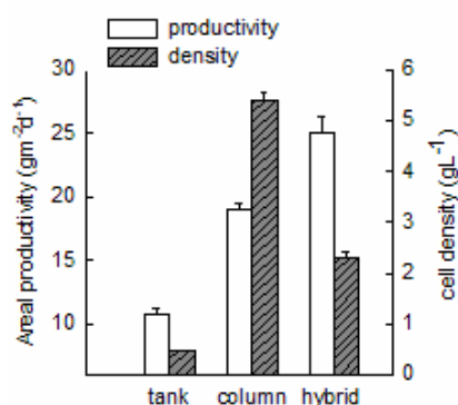
Fig.4: Maximum cell density and average areal productivity in various cultivation systems (tank, column, and hybrid).
