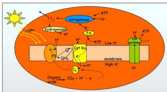
Figure 2: Photofermentation in a purple non sulfur bacterium. PS = photosystem; Fd = ferredoxin; Cyt bc 1 = Cytochrome bc 1 ; c 2 = Cytochrome c 2 .
