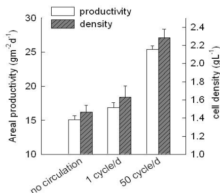
Fig.7: Effect of hybrid system on maximum biomass density and average areal productivity in a batch culture.
