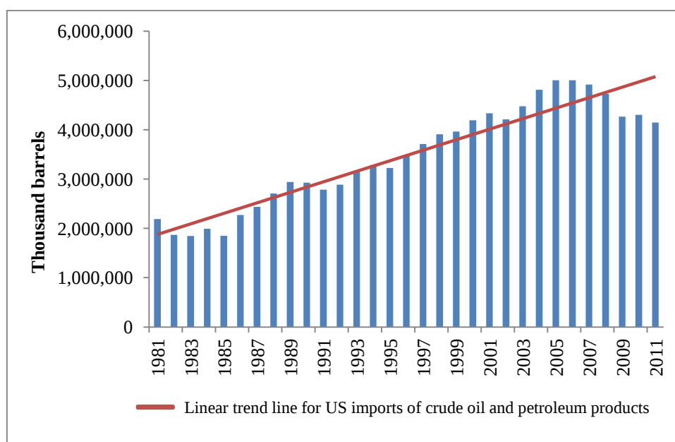
Figure 2.2.1 US imports of crude oil and petroleum products
