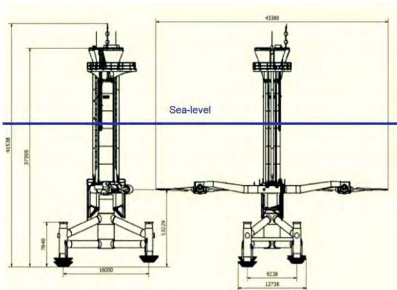
Figure 14. SeaGen layout
