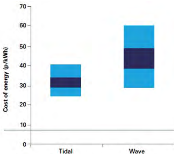
Figure 37. Baseline costs for benchmark first farm wave and tidal devices. These costs assume a discount rate of 15% and a lifetime of 20 years. The dark bars represent CoE at medium energy (upper bound) and high energy (lower bound) sites, using base case cost and performance assumptions; while the outer bars add optimistic and pessimistic cost and technical assumptions to these limits
