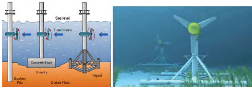
Figure 2. Tidal current devices
