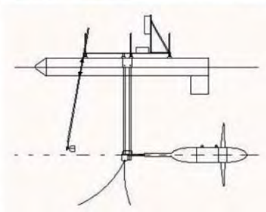
Figure 10. World's first tidal current turbine
