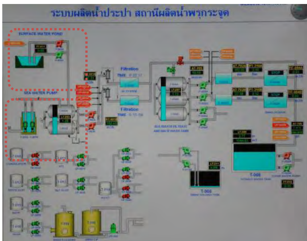
FIGURE 13-5 : Water Treatment Plant Process at Krajud.
