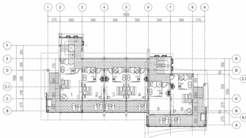
FIGURE 11-27 : Typical Room Floor Plan for Hotel
