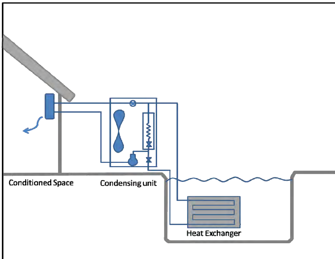
FIGURE 11-6 : Hybrid split type system
