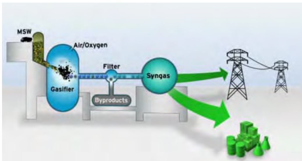
FIGURE 10-2 : Gasification Process
