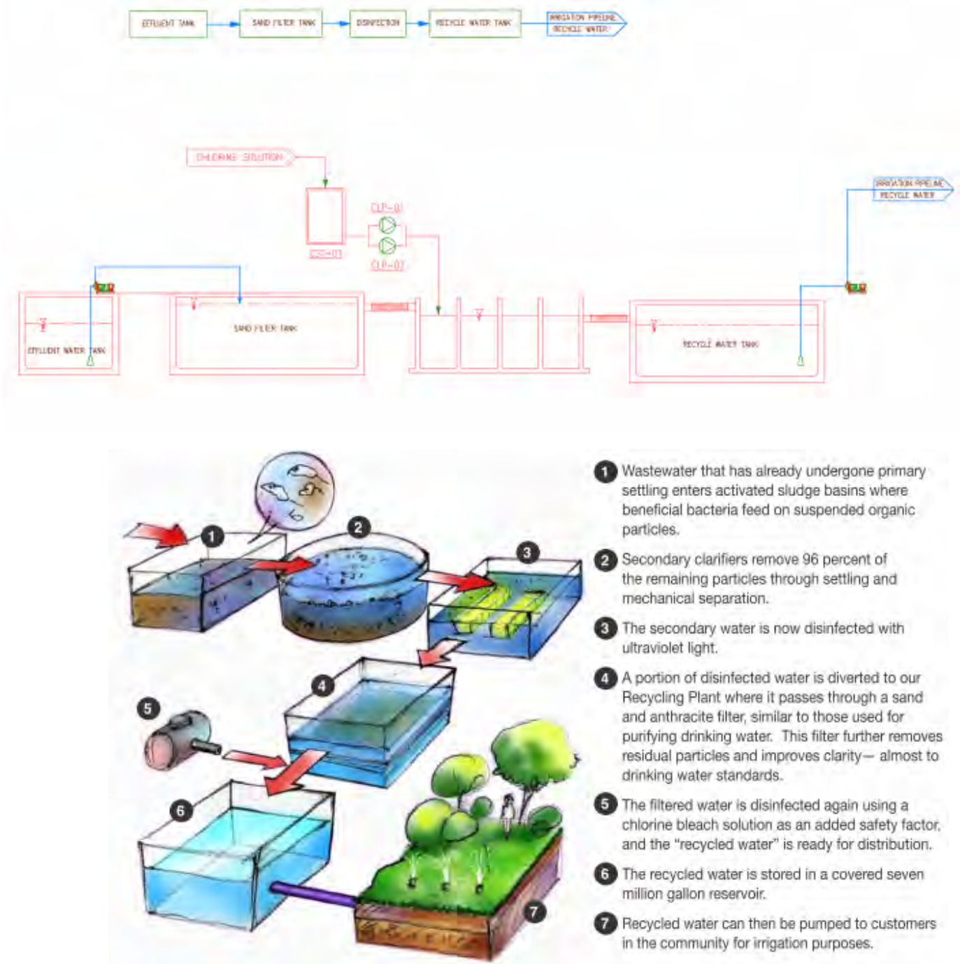
FIGURE 13-10 : Flow Diagram for Recycled Water Treatment Process System
