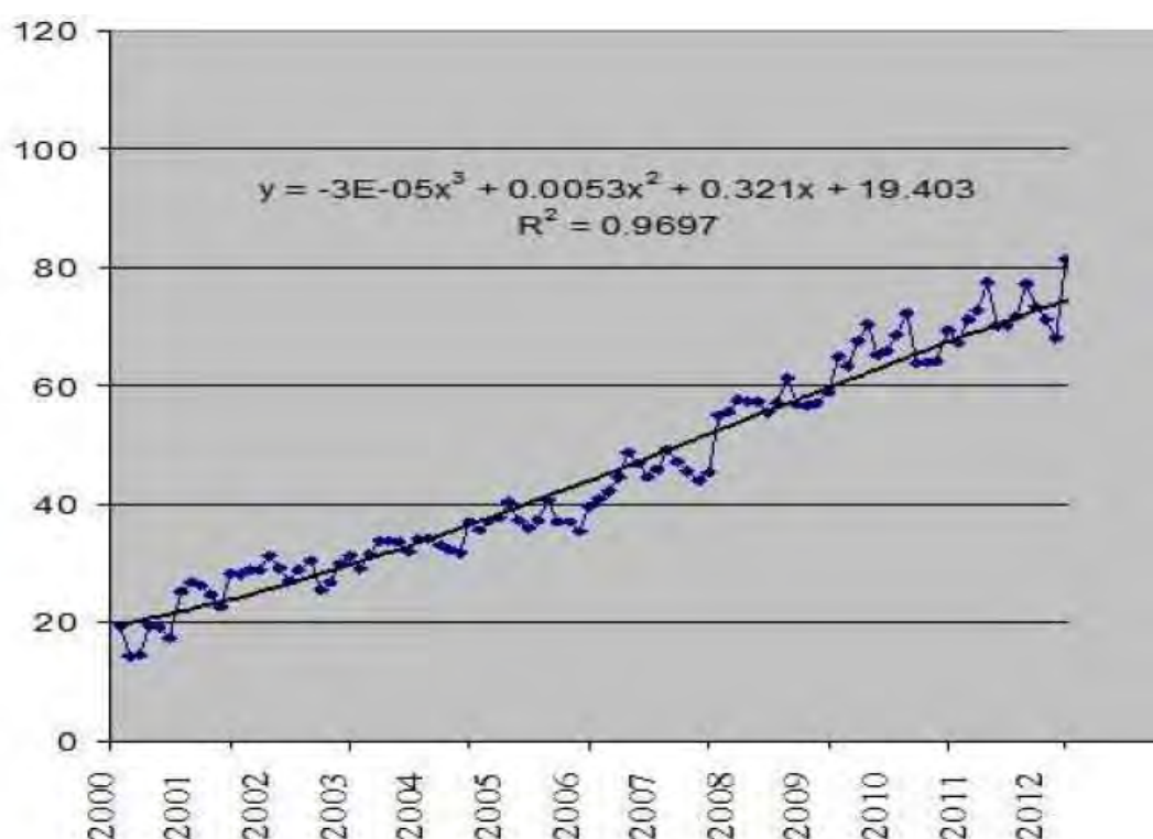
FIGURE 8-3 : Electrical peak demand equation created by using historical data
