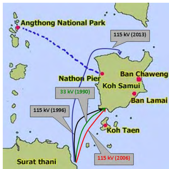
FIGURE 2-2 Existing Submarine Cable for electrical power supply
