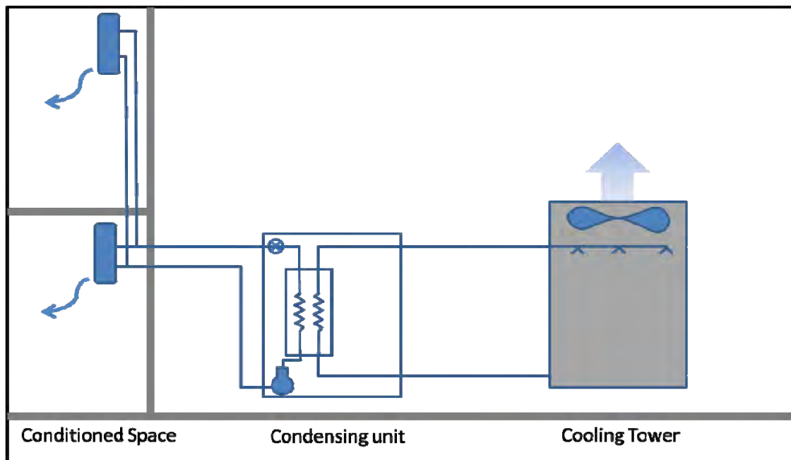
FIGURE 11-8 : Water-cooled Variable Refrigerant Flow (VRF) system
