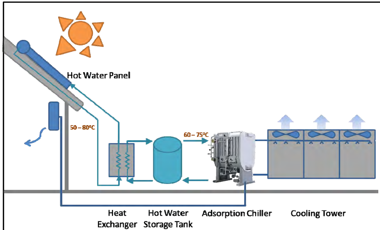
FIGURE 11-9 : Adsorption chiller system
