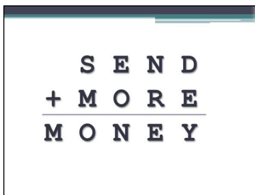
Fig IV.1: A cryptarithm
